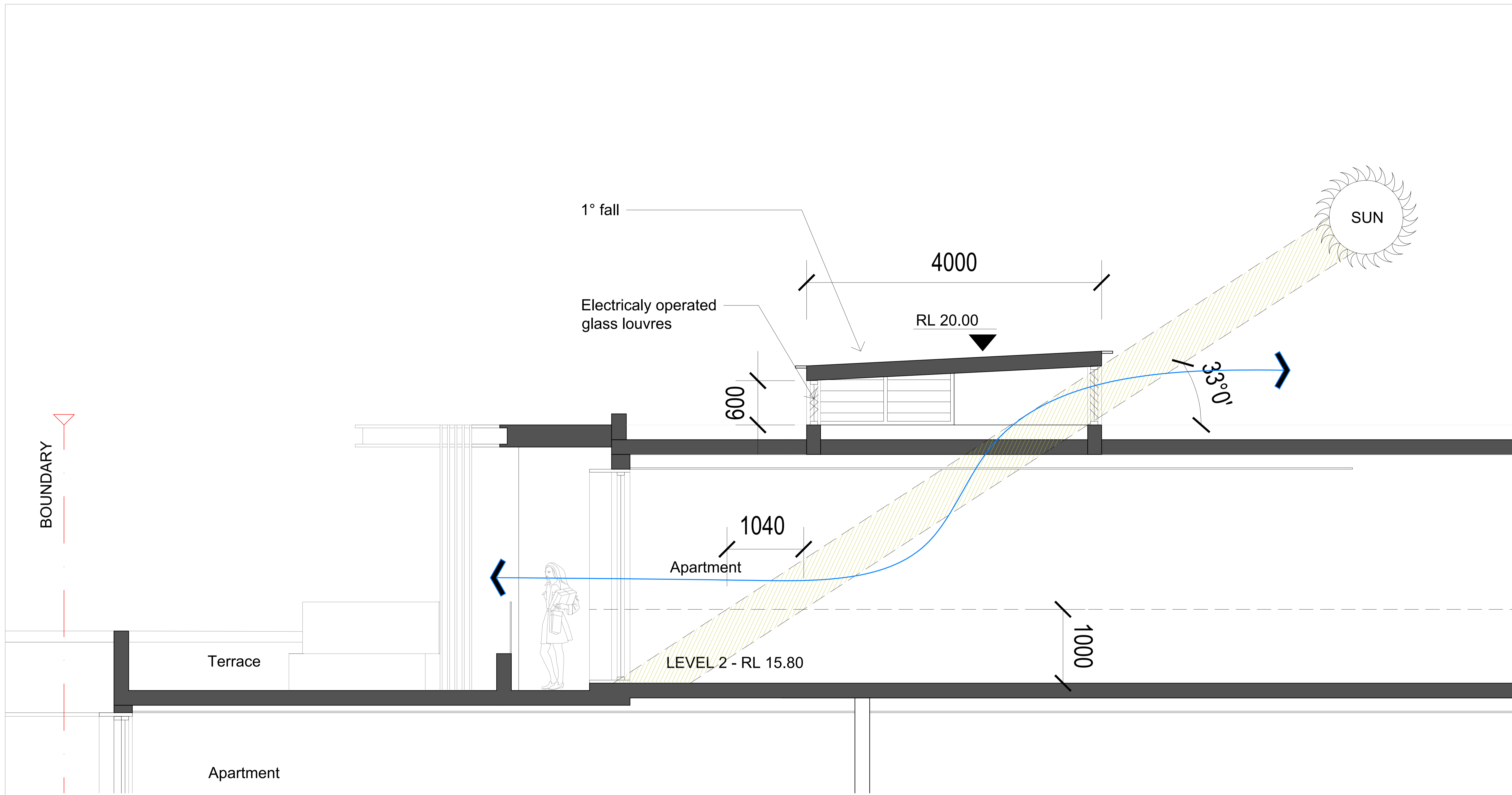
01 TYPICAL SKYLIGHT SECTION SCALE- 1:50 @ A1
